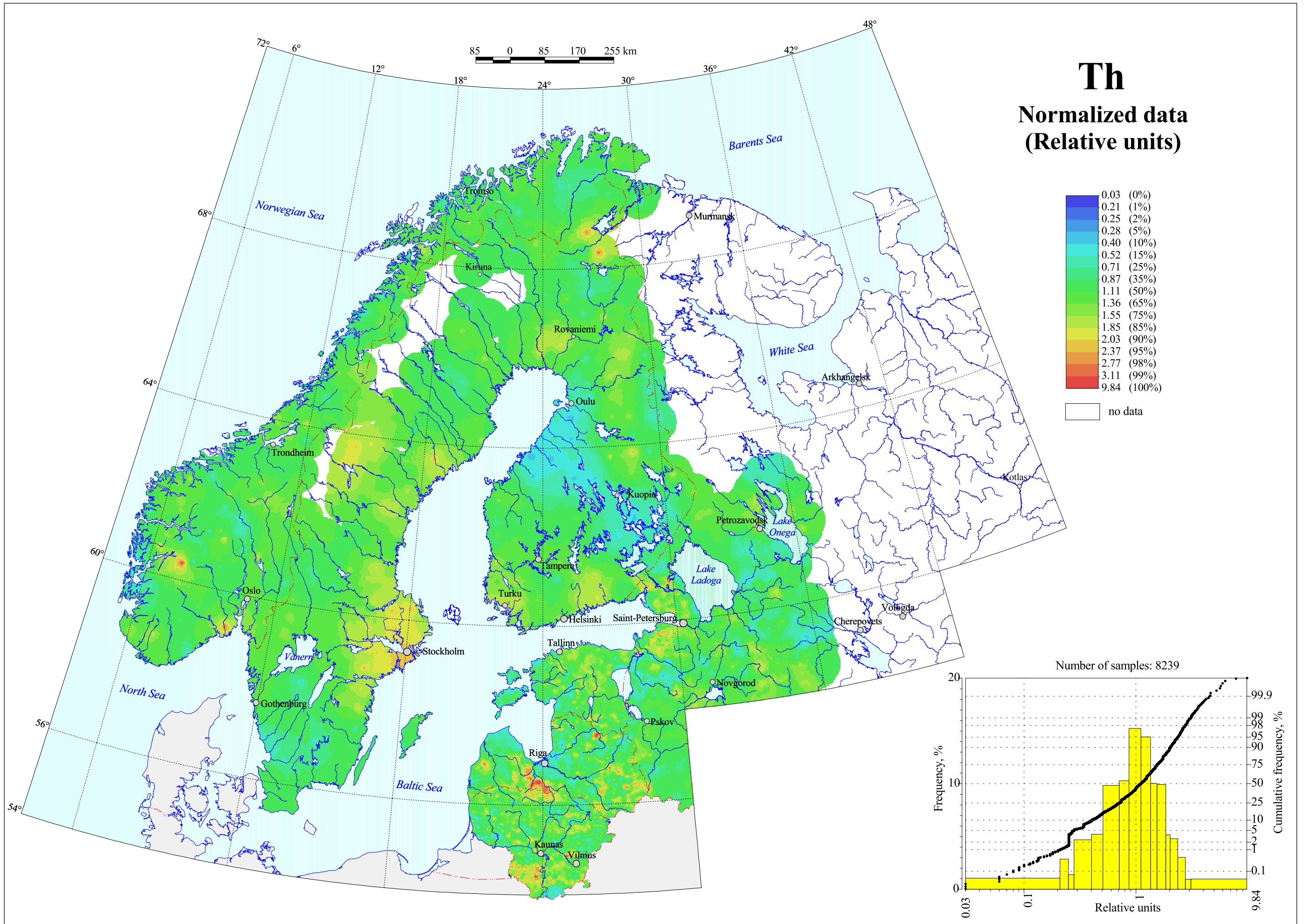
Thorium in Topsoil
